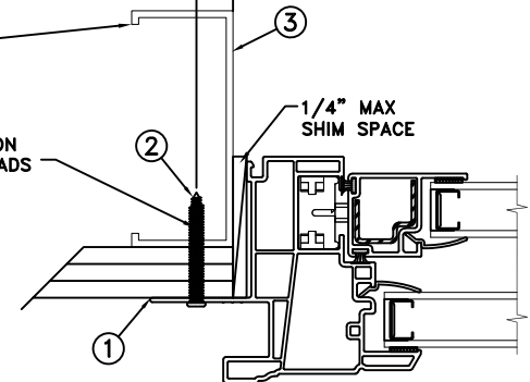
FRAME JAMB SECTION (TYP) HORIZONTAL SECTION
